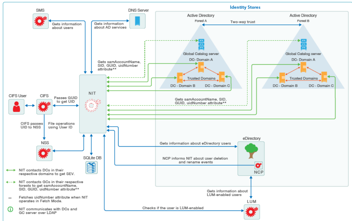
Figure 7-1 NIT - overview
