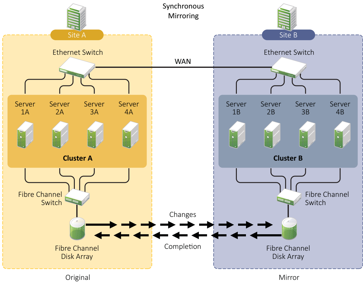
Figure 1-2 Cluster of Clusters with Storage-Based Data Mirroring
