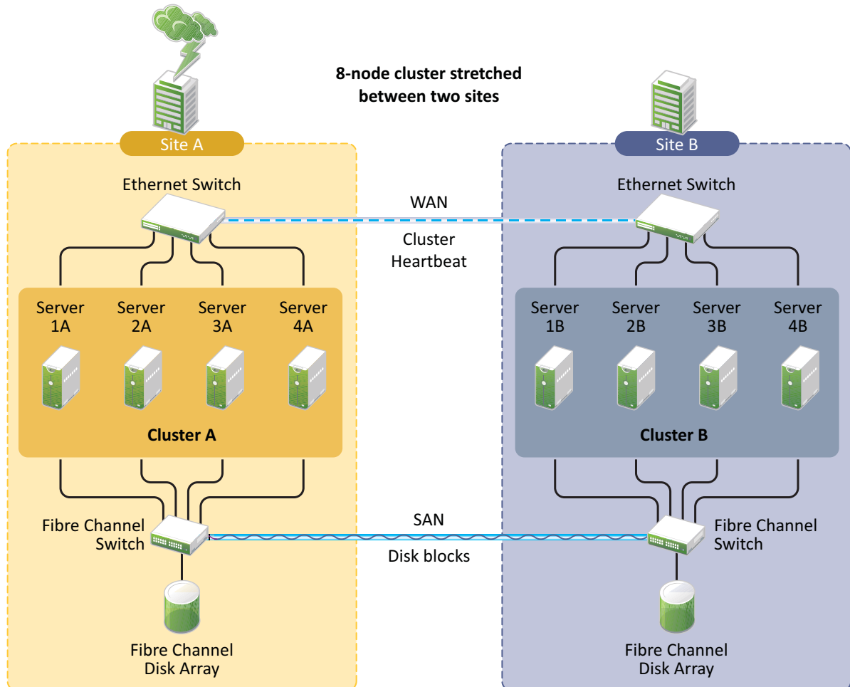
Figure 1-1 Stretch Cluster
