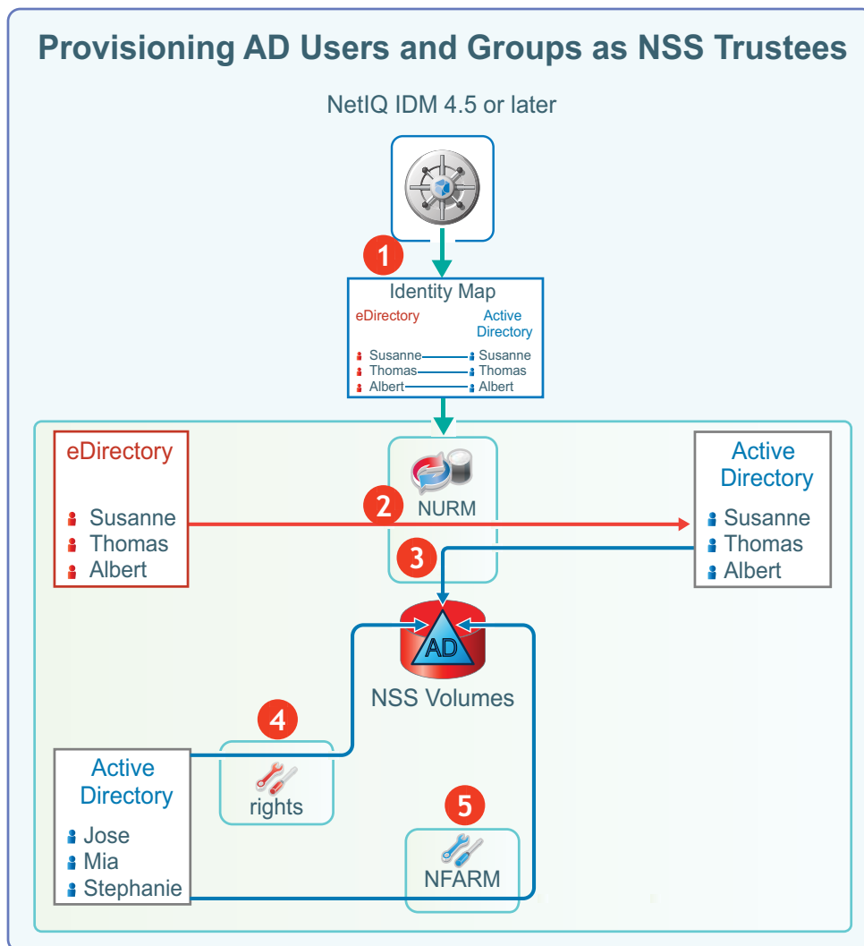
Figure 5-1 Provisioning AD User and Groups for NSS Access
