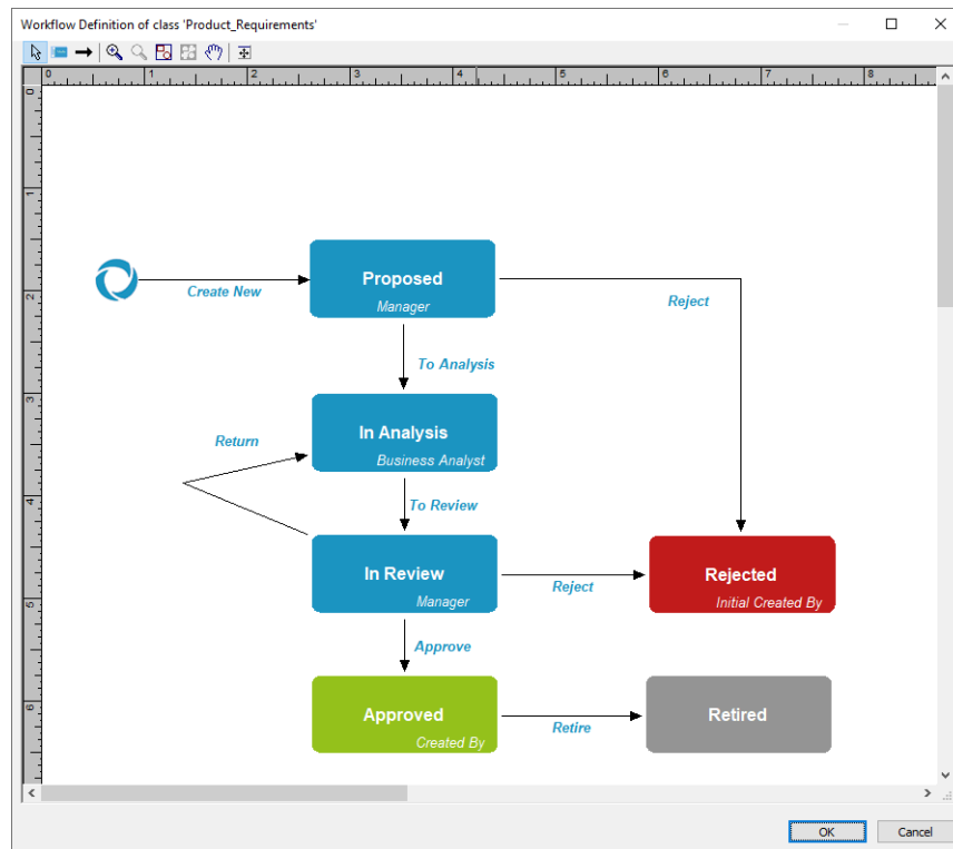
Figure 9-26. Workflow for class Product_Requirements
