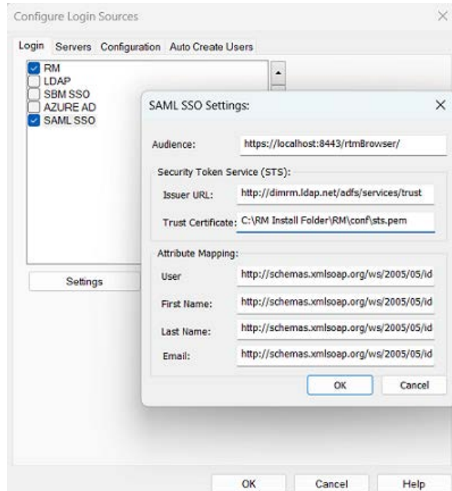
Figure 4-5. Configure SAML SSO Login
